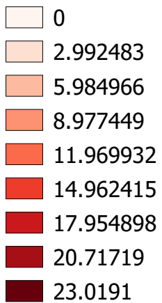
Heatmap
